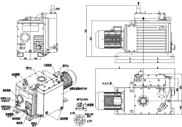
BSF120B - DRV175Y/275Y
