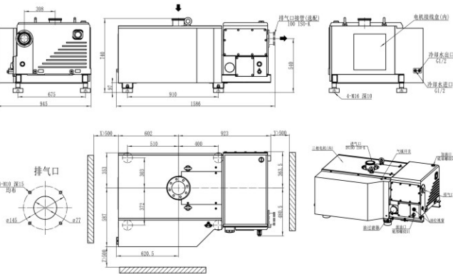
SRV630W/750W
