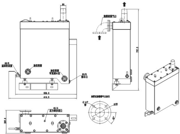
BSF120B
