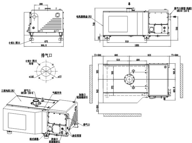
SRV630A/750A
